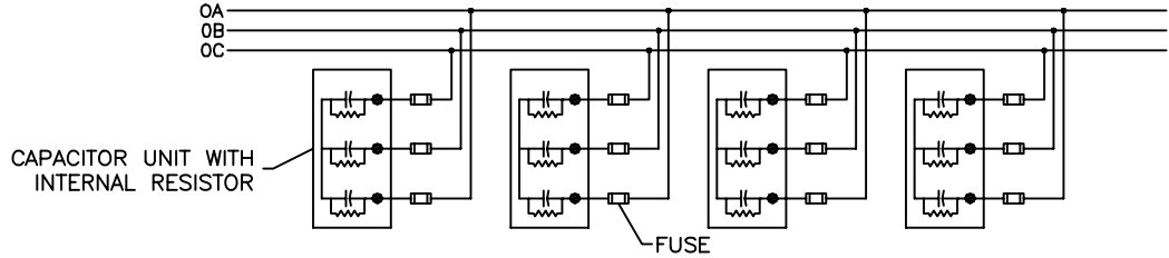
CONNECTION DIAGRAM
