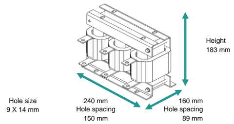
Preliminary dimensions
