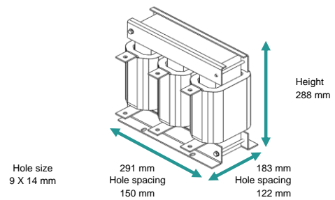
Preliminary dimensions
