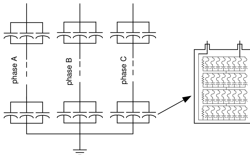
Fig.3. Internally fused shunt capacitor bank and capacitor unit.
