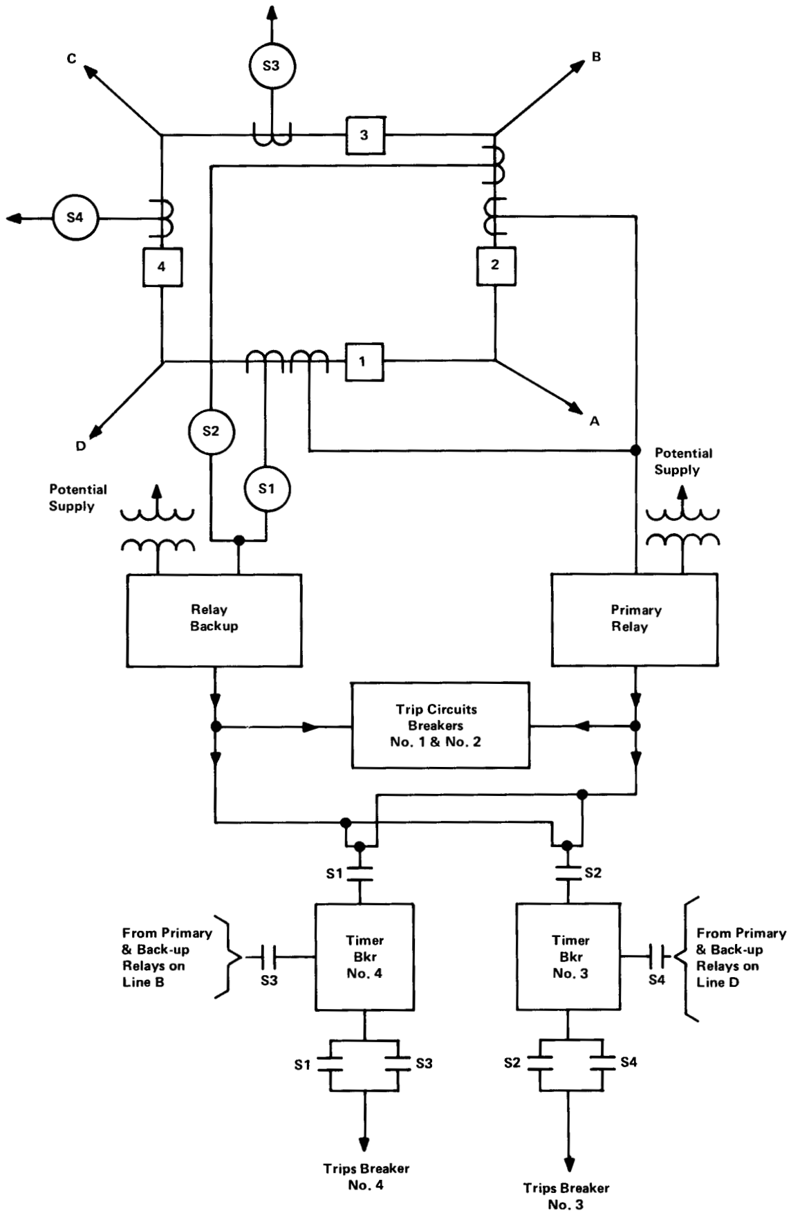
Fig. 4. Proposed back-up scheme for a line connected to a ring bus
