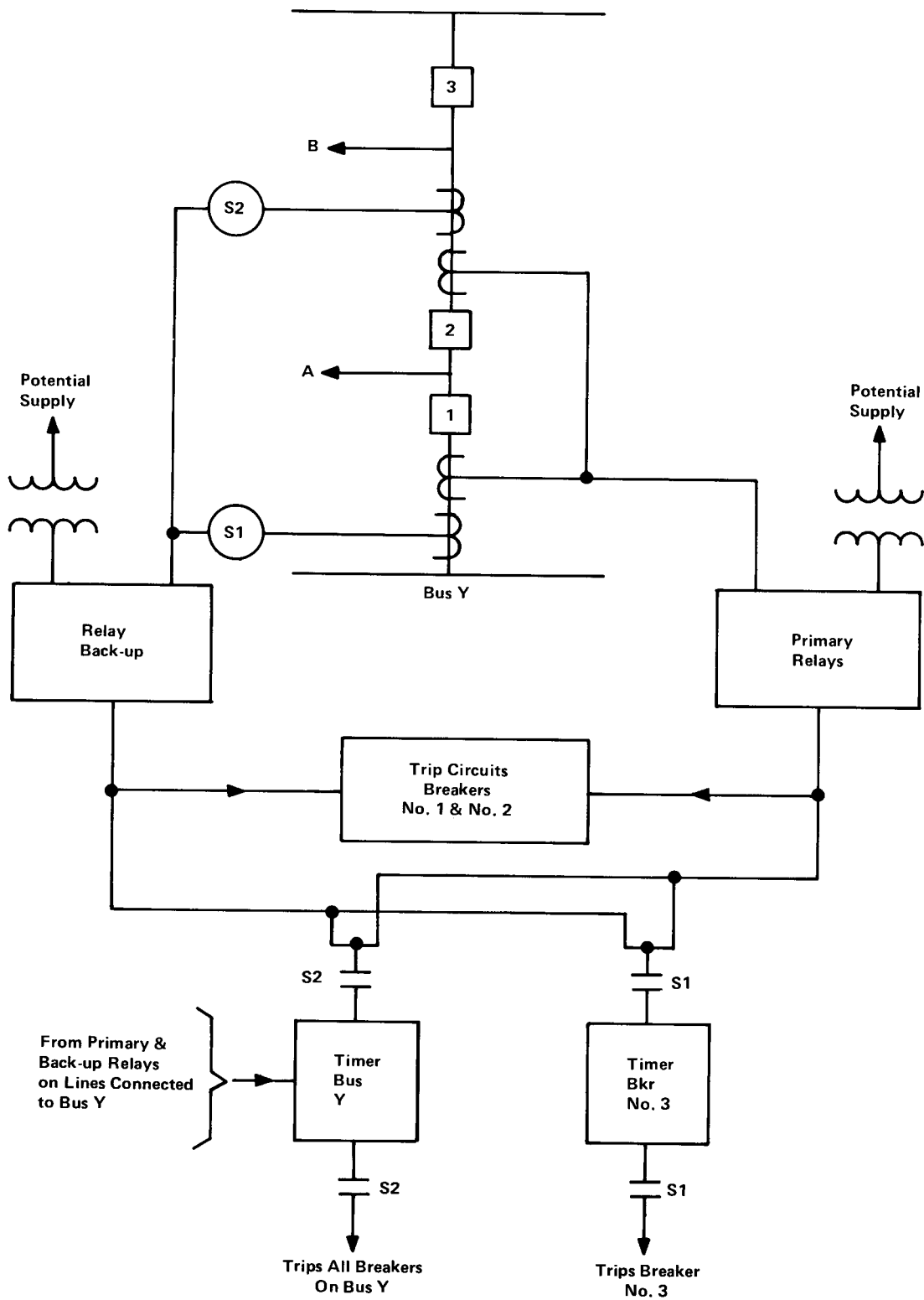
Fig. 3. Proposed back-up scheme for a line connected to a breaker-and-a-half arrangement
