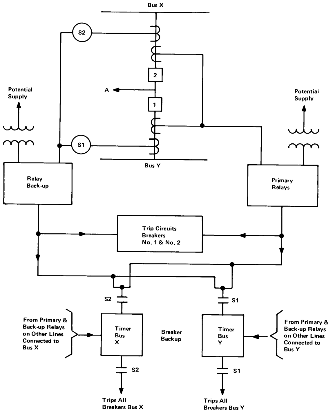
Fig. 2. Proposed back-up scheme for a line connected to a double bus-double breaker arrangement
