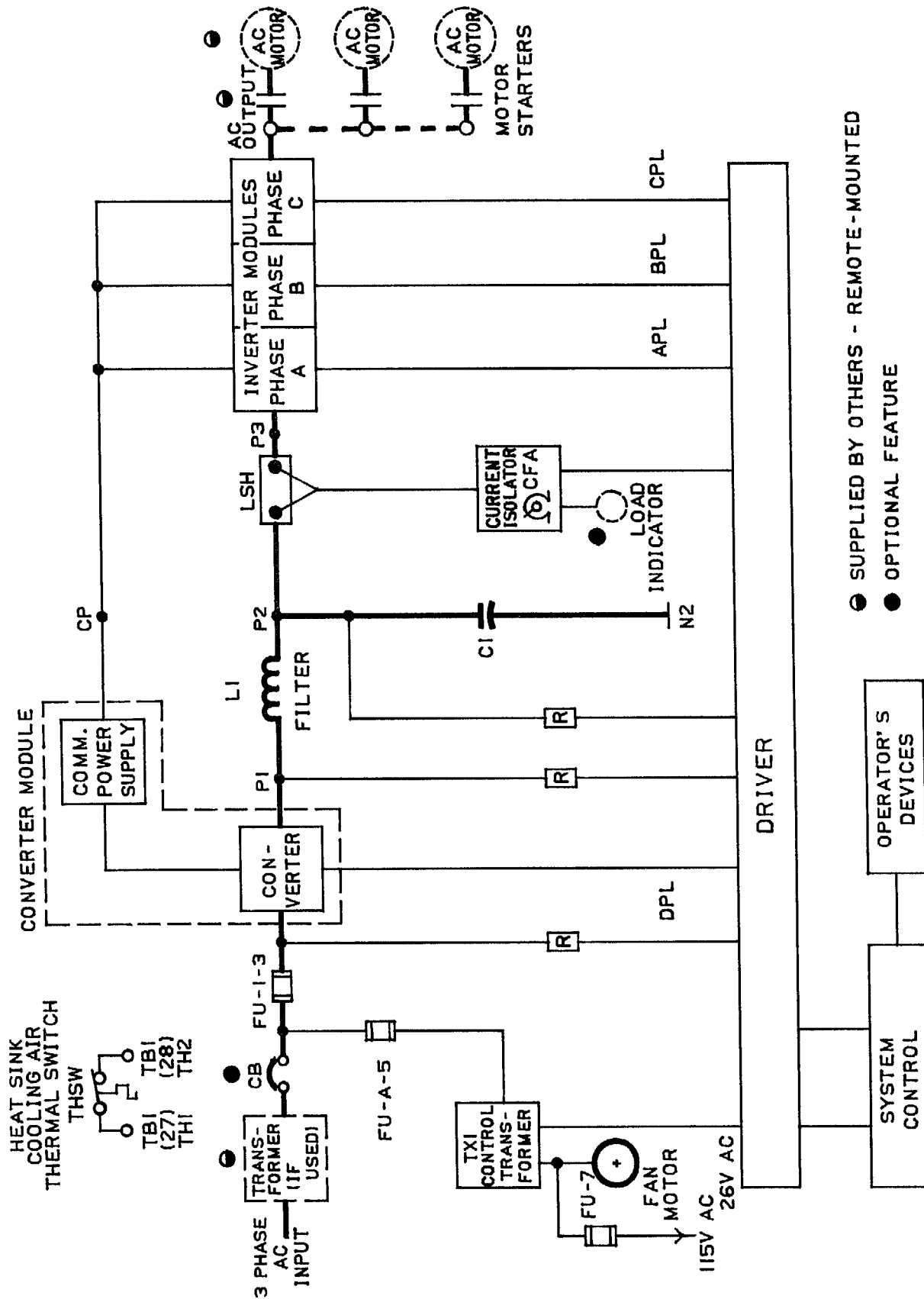
FIG. 2 AF-400 DRIVE SYSTEM BLOCK DIAGRAM
