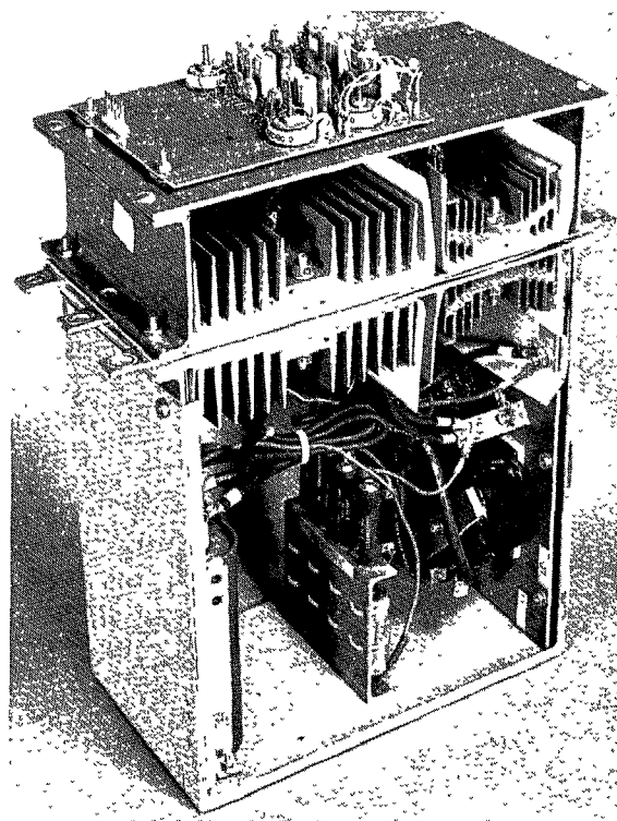
FIGURE 22 AF-400 Drive Inverter Phase Module standing on a table stud mounted SCRs 10-30 KVA, 230 or 460V AC (Photo MG-5629-11)
