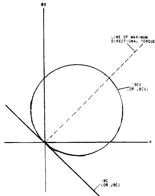
Fig. 6 Impedance Characteristics Of The Type JBC And JBCV Relays
