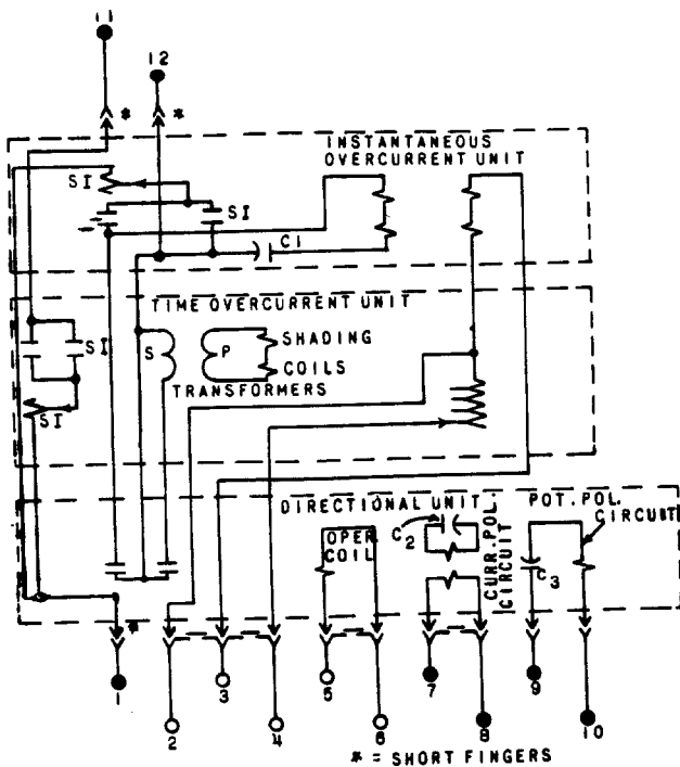
Fig. 19 Internal Connections For The Type JBC651M Relay (Front View)
