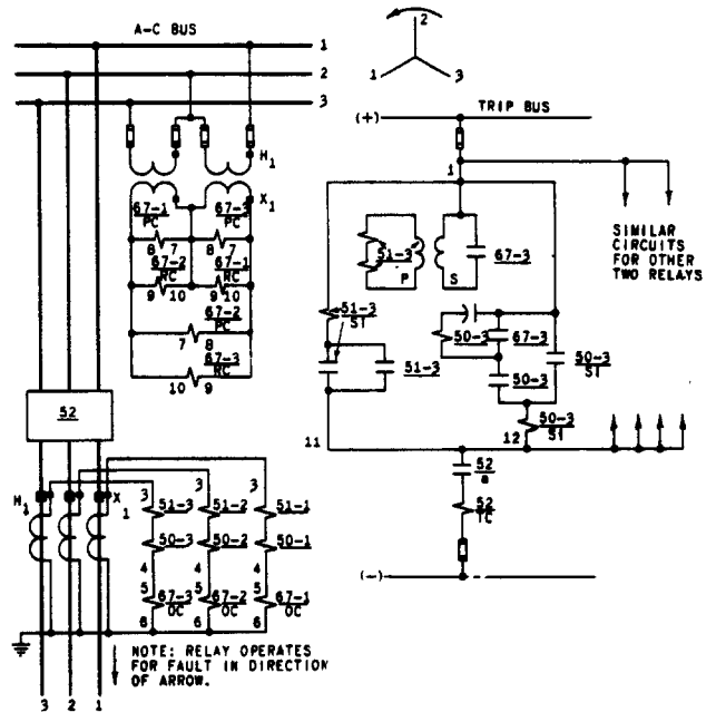
Fig. 4 Typical External Connections For Directional Overcurrent Protection Of A Line Using Three Type JBCV51M Relays
