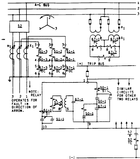
Fig. 2 The 90-Degree Connection Three Type JBC51M Relays Used For The Directional Overcurrent Protection Of A Single Line
