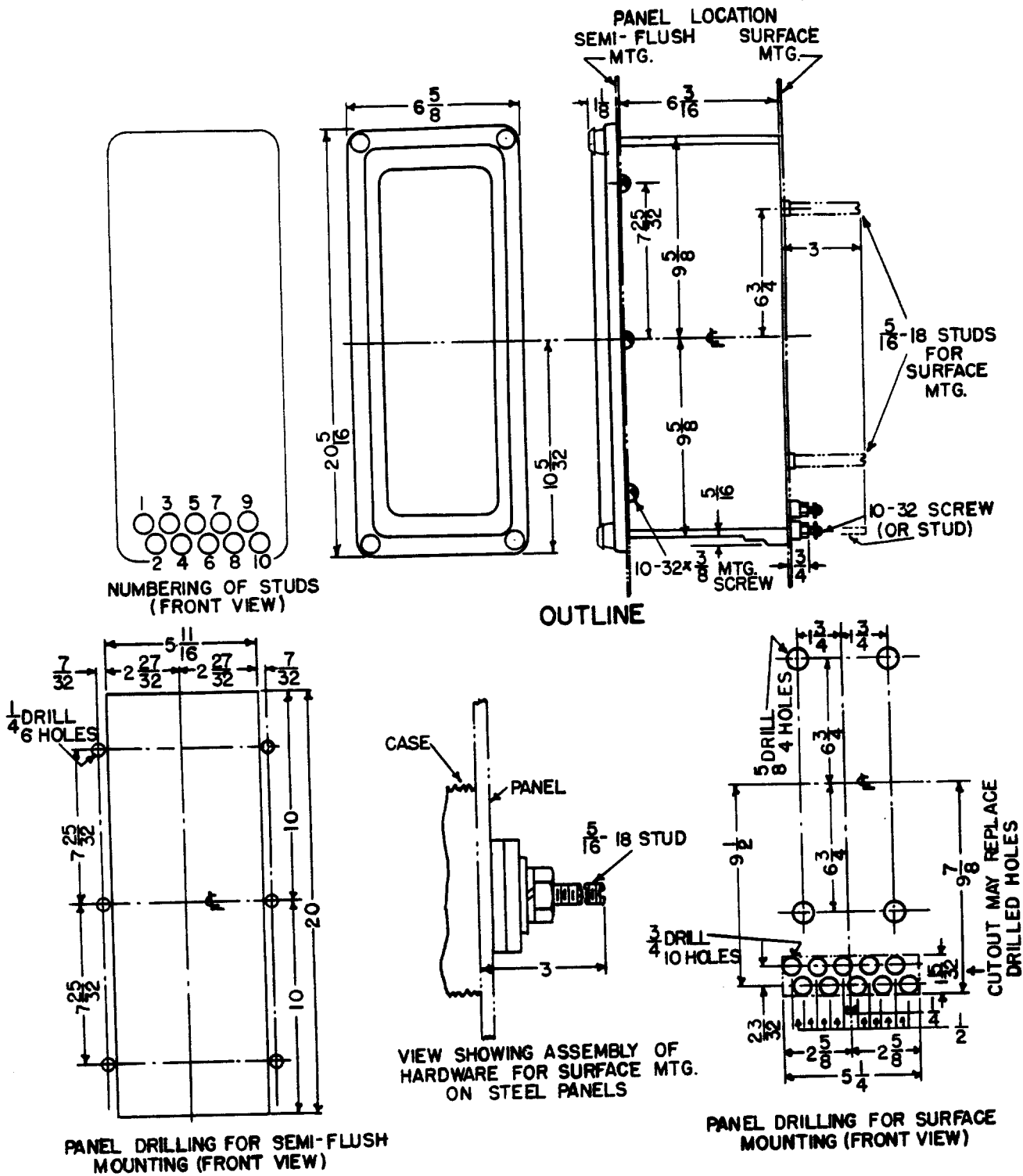
Fig. 26 Outline And Panel Drilling Dimensions For The Type JBC51N Relay
