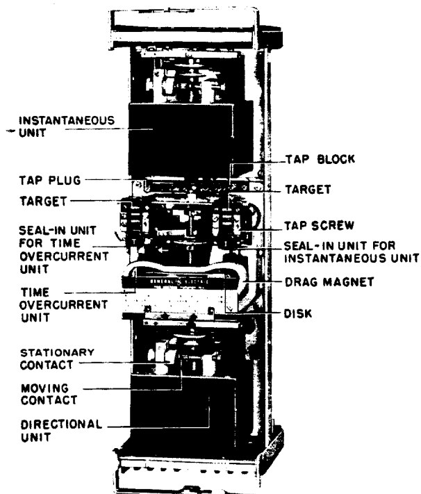
Fig. 15 Type JBCV5IN Relay-Unit In Cradle (Front View)
