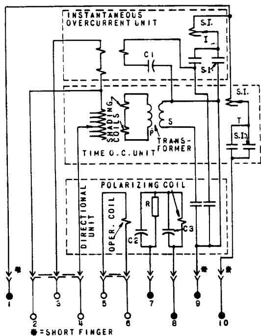
Fig. 17 Internal Connections For The Type JBC5IN Relay (Front View)
