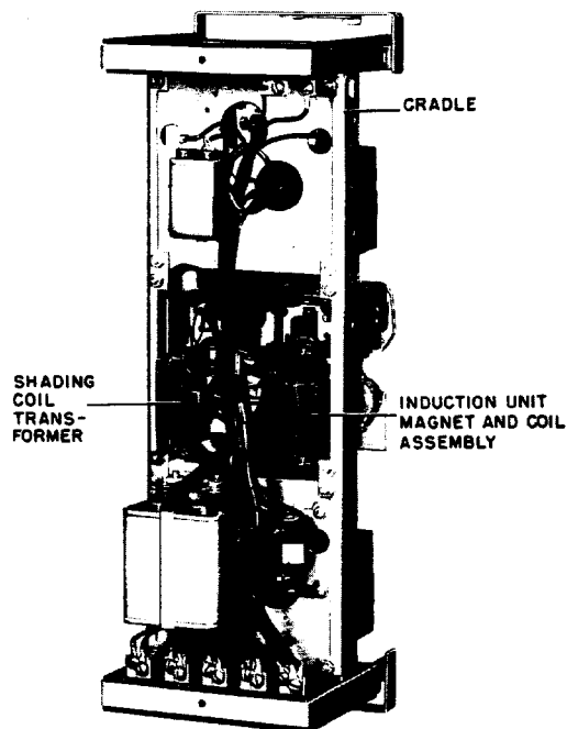
Fig. 16 Type JBCV5IN Relay-Unit In Cradle (Rear View)
