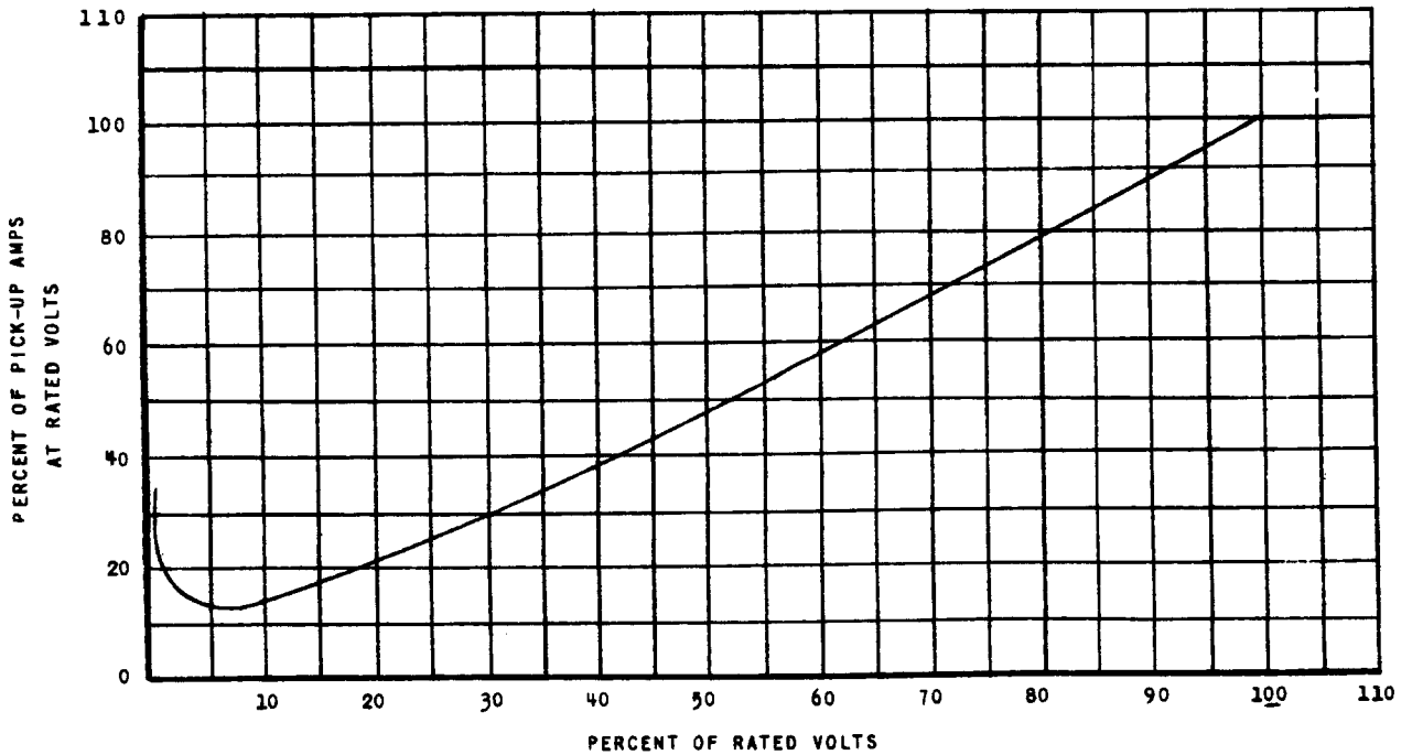
Fig. 8 Typical Directional Unit Pick-up Characteristics Of The Type JBCV Relay With Balanced Voltages And At Maximum Torque Angle
