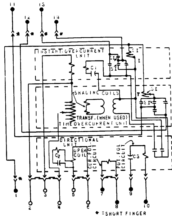
* Fig. 20 Internal Connections For The Type JBC652M Relay (Front View)
