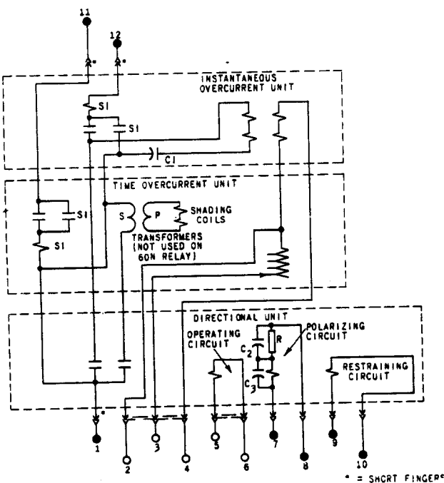
Fig. 21 Internal Connections For The Type JBCV51M Relay (Front View)
