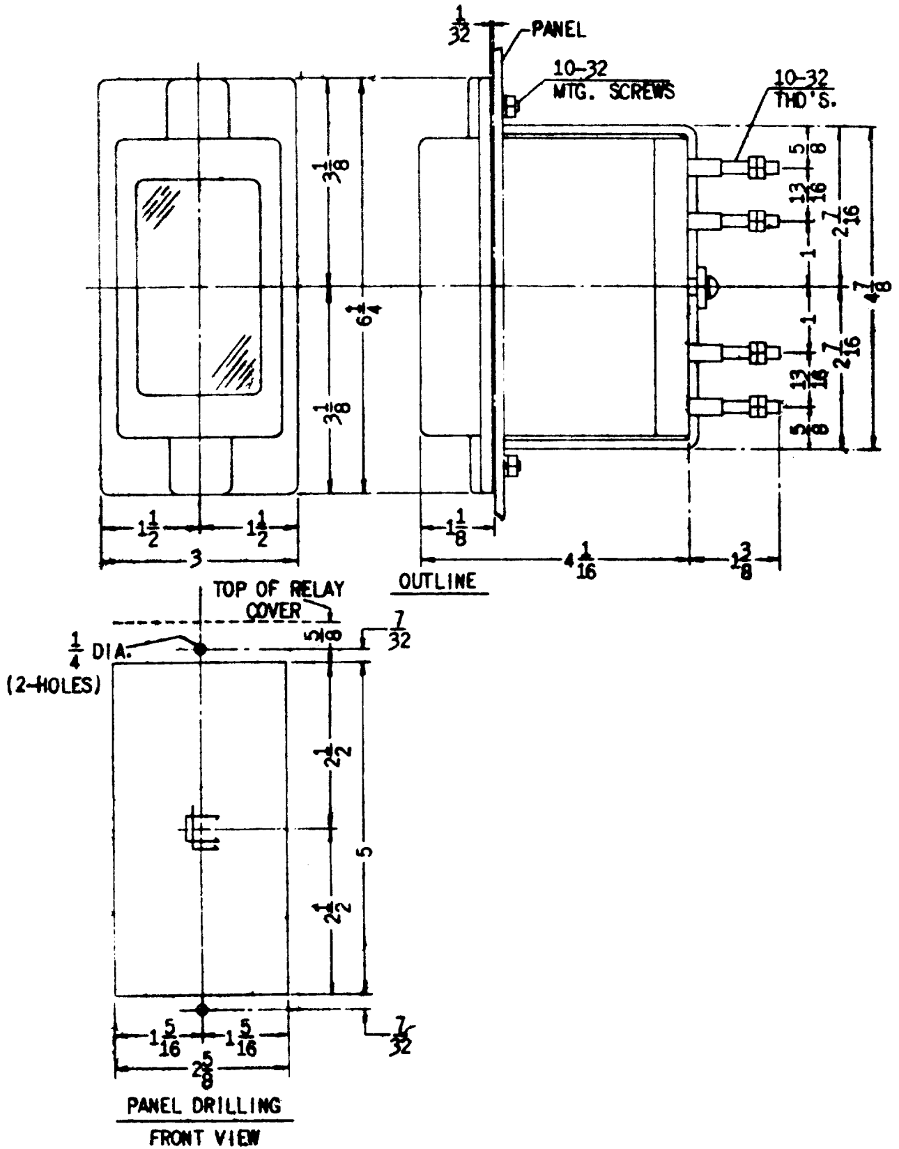
Fig. 4 (0148A3978-2) Outline and Panel Drilling Dimensions for the Semi-flush Mounted NLA15A Relay
