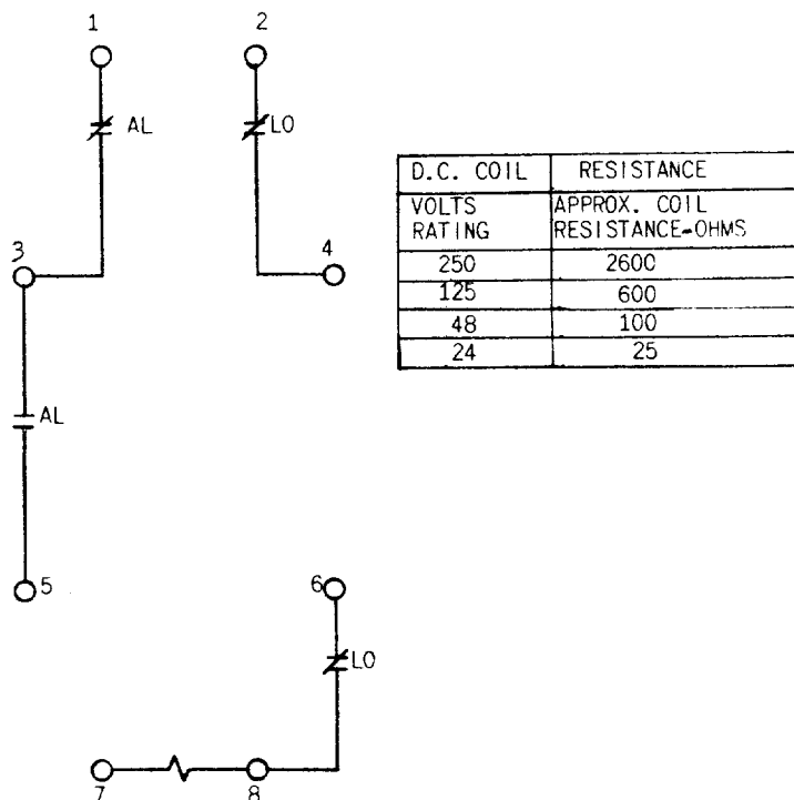
Fig. 3 (0165A7604-1) Internal Connection Diagram (Back View) of the NLA15A Relay
