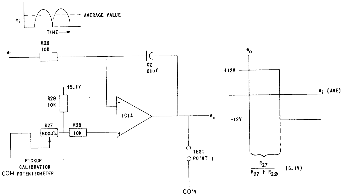
FIGURE 3. (0257A5010-2) RECTIFIER AND TAP RESISTORS
