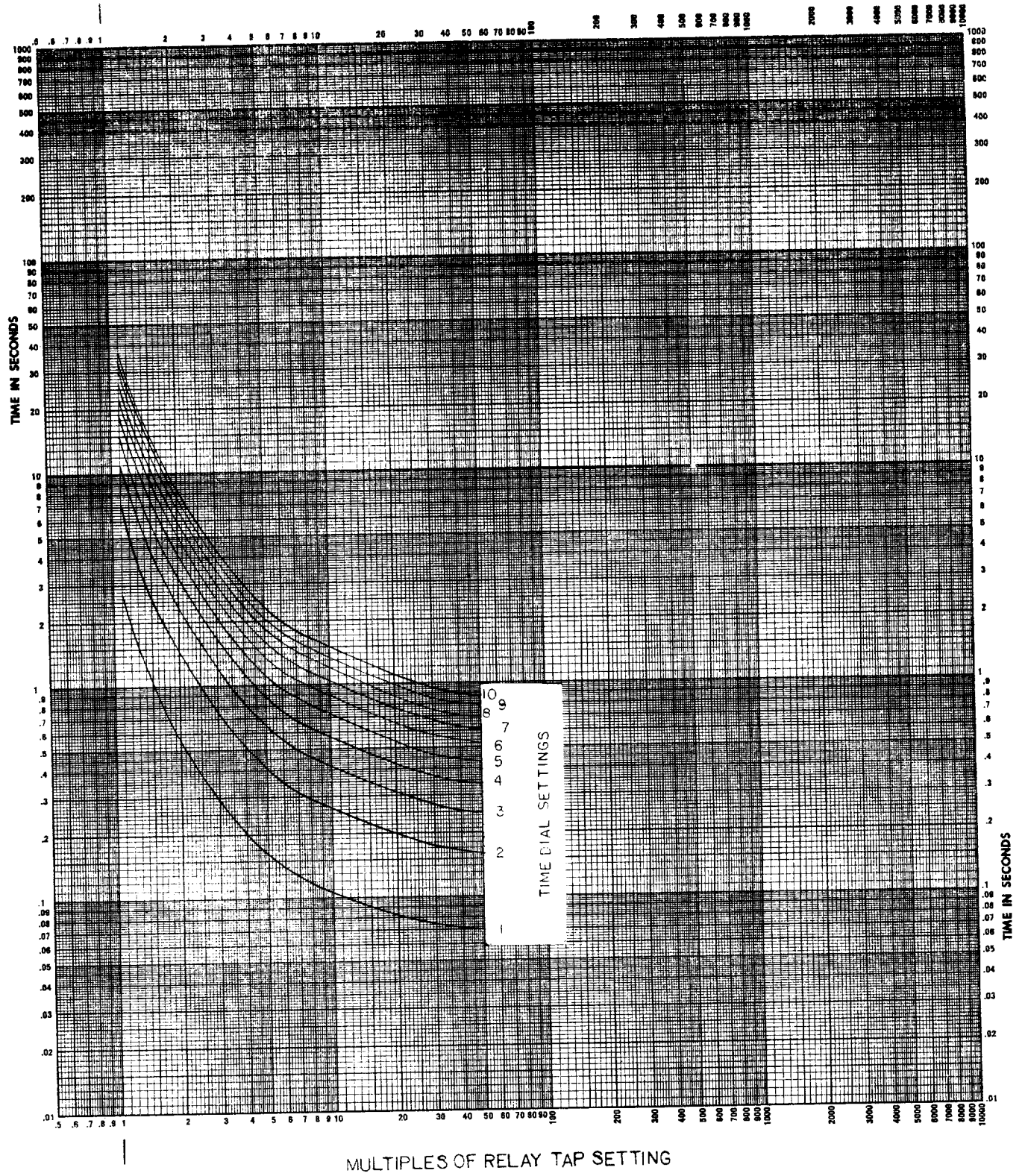
FIGURE 16. (0183B7888-3) TIME-CURRENT CURVES SFC TIME-OVERCURRENT RELAY TYPE - VERY INVERSE
