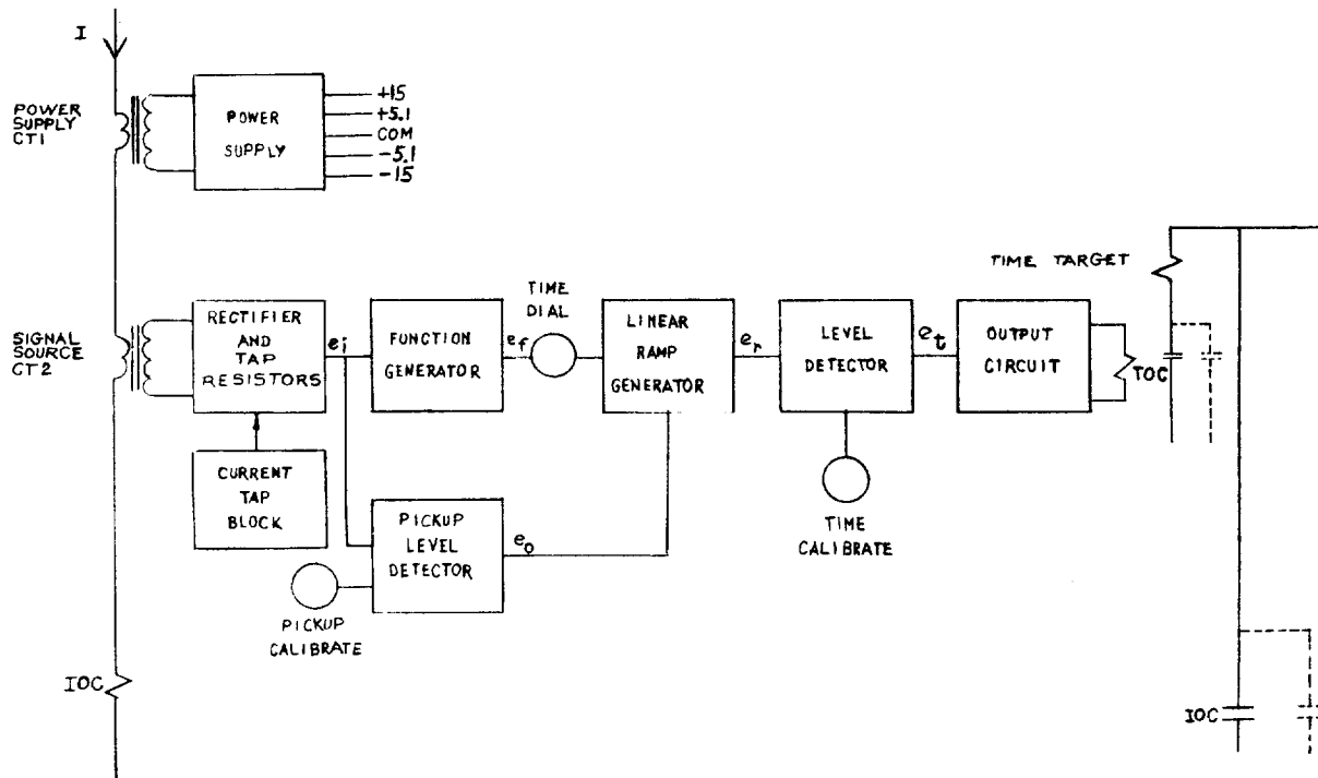
FIGURE 2. (0257A5009-1) FUNCTIONAL BLOCK DIAGRAM OF THE SFC RELAY
