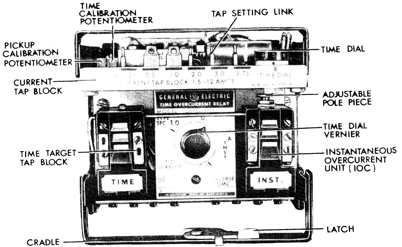
SFC RELAY - FRONT VIEW (REMOVED FROM CASE)
