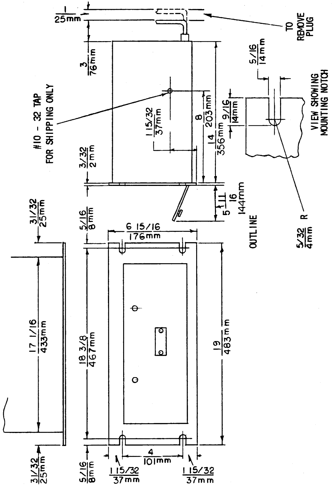
Fig. 4 (0227A2037-0) Outline and Mounting Dimensions
