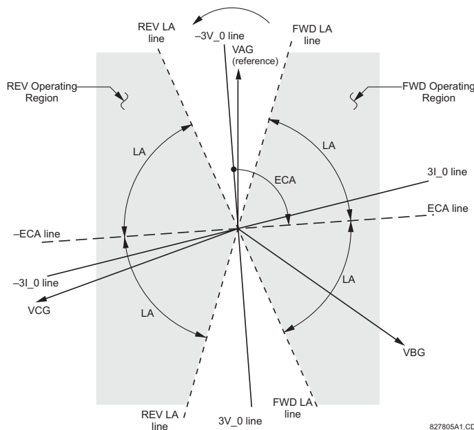
Figure 5-51: NEUTRAL DIRECTIONAL VOLTAGE-POLARIZED CHARACTERISTICS
