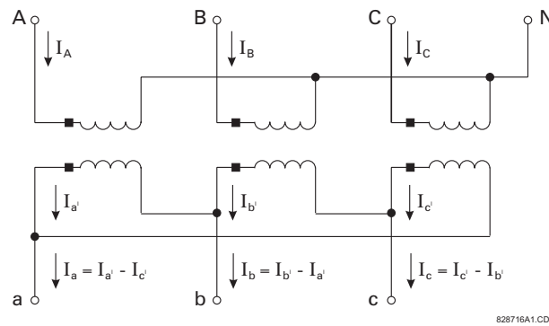
Figure 5-14: EXAMPLE TRANSFORMER
