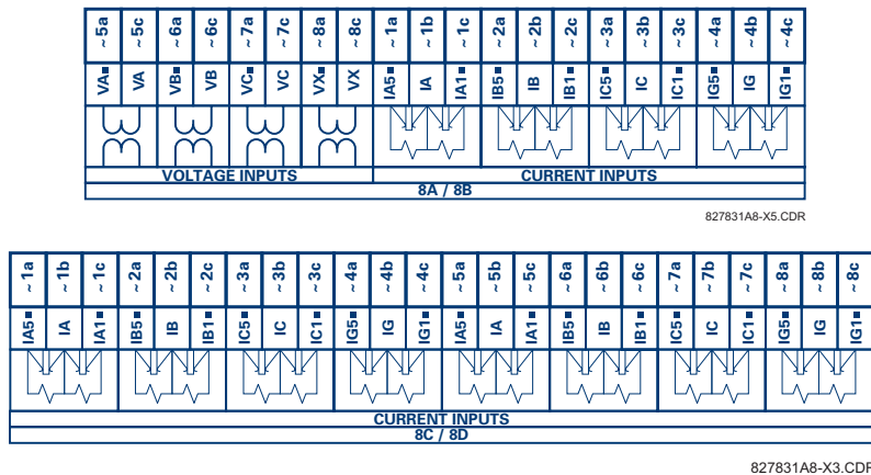
Figure 3-11: CT/VT MODULE WIRING
