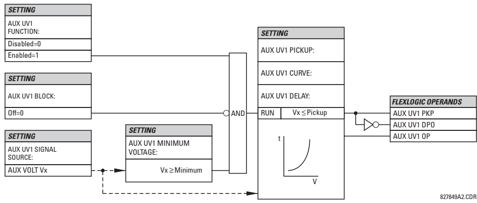
Figure 5–62: AUXILIARY UNDERVOLTAGE SCHEME LOGIC
