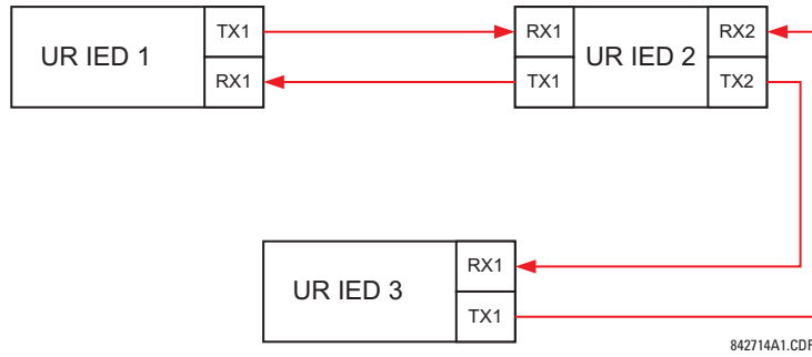
Figure 5-80: SINGLE-CHANNEL OPEN-LOOP CONFIGURATION
