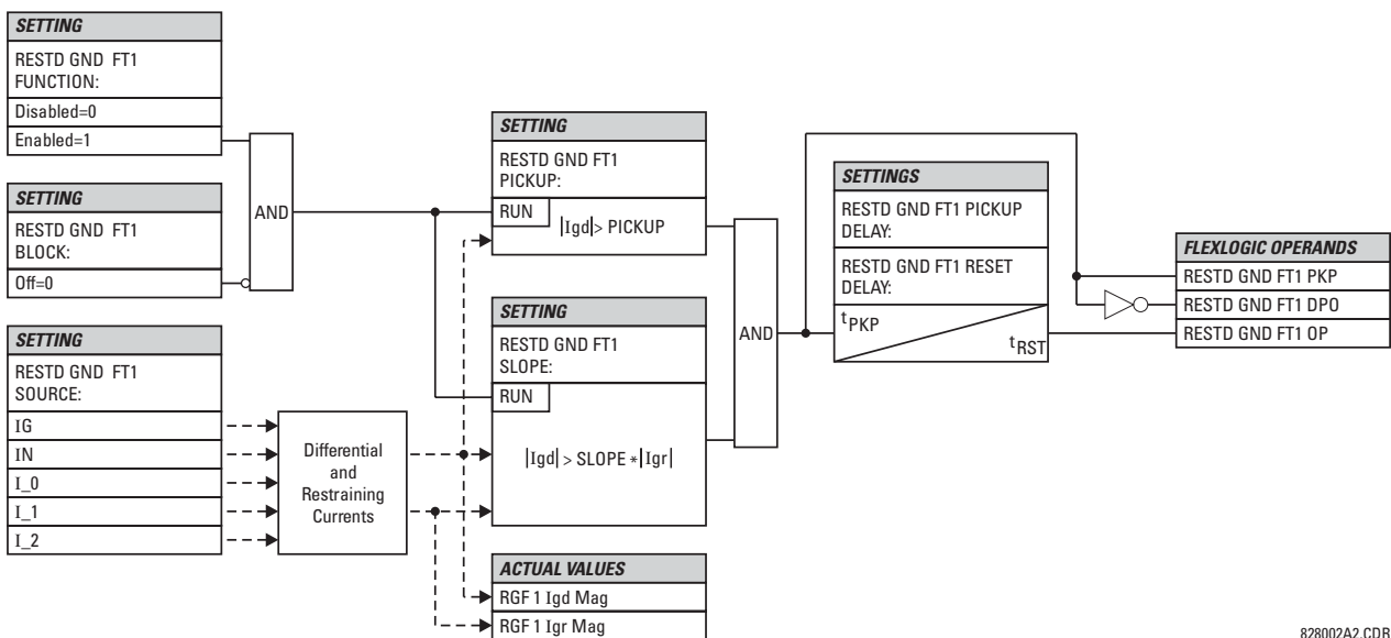
Figure 5-57: RESTRICTED GROUND FAULT SCHEME LOGIC
