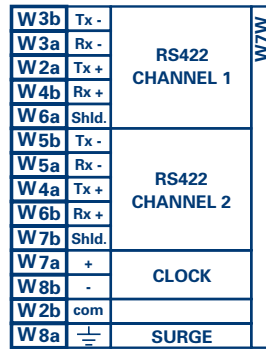
RS422.CDR p/o 827831A6.CDR
