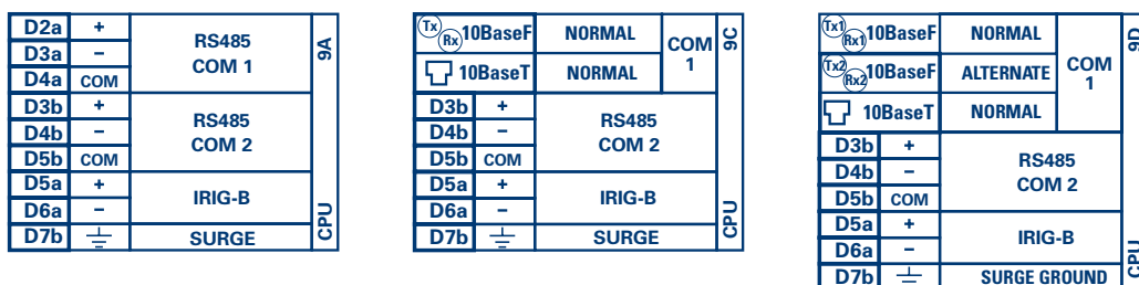
Figure 3-18: CPU MODULE COMMUNICATIONS WIRING
