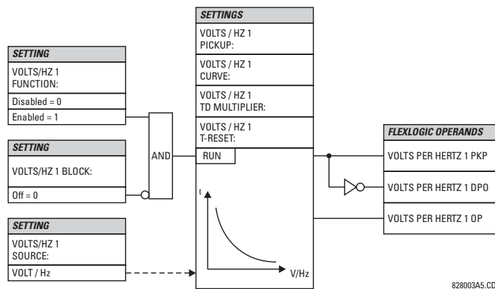
Figure 5-64: VOLTS PER HERTZ SCHEME LOGIC
