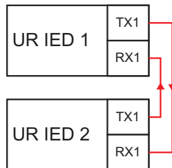
Figure 5–77: INPUT/OUTPUT EXTENSION VIA DIRECT I/Os
