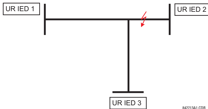
Figure 5-79: THREE-TERMIAL LINE APPLICATION
