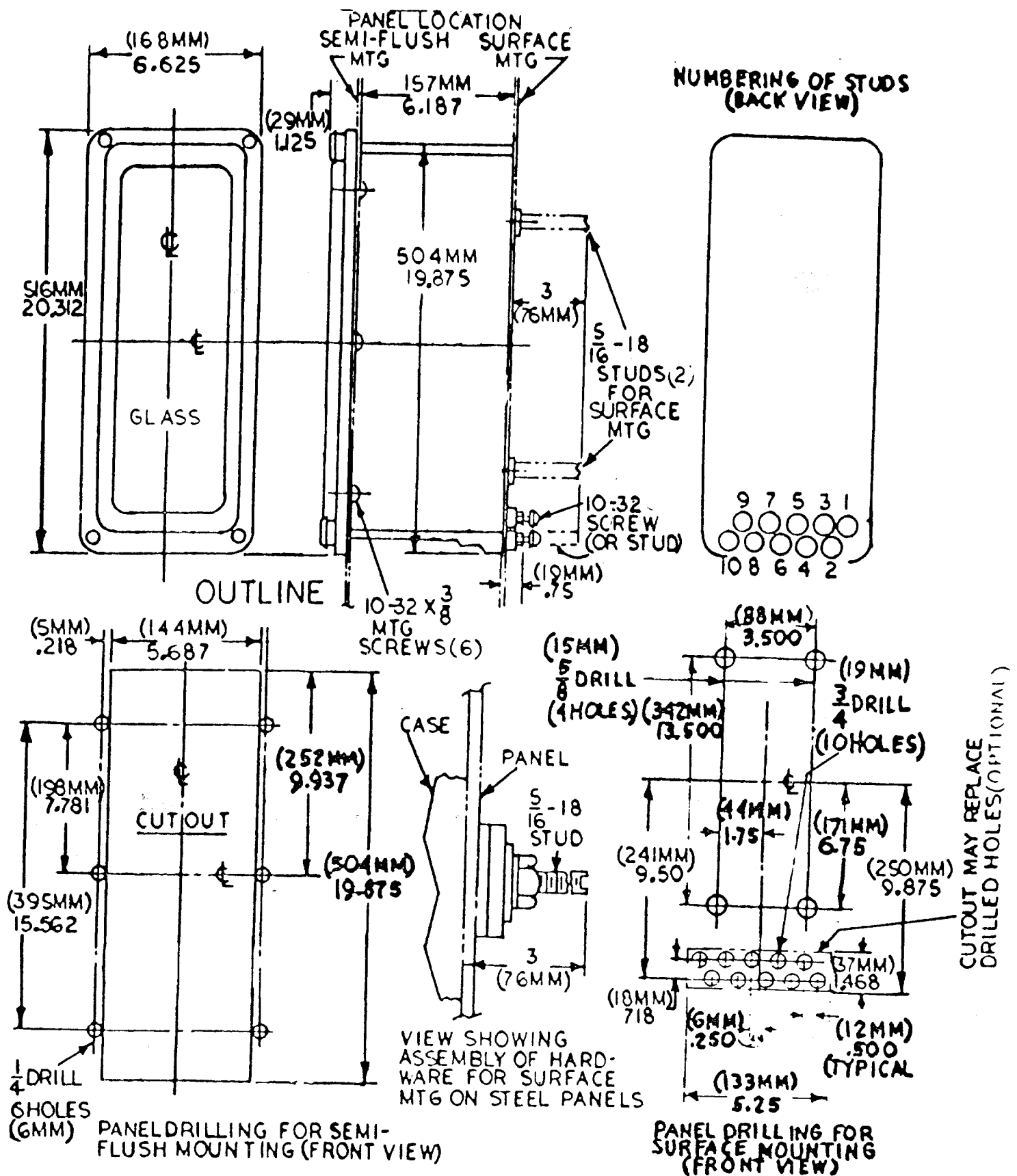
Fig. 12 (6209275-3) Outline and Panel Drilling Dimensions for Relay Types IJC51B and IJC53A
