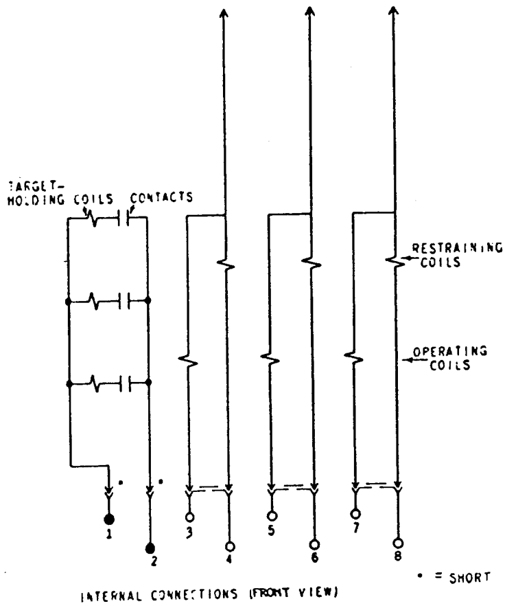
Fig. 7 (6306693-3) Internal Connections for Relay Types IJC51B and IJC53A (Front View)
